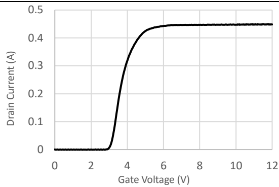
Figure 13. Transfer characteristics at V_{DS} = 0.1 \text{ V} , T_J = 25 \text{ }^{\circ}\text{C} .
