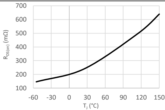
Figure 12. On-state resistance as a function of junction temperature at V_{GS} = 12\text{ V} and I_D = 0.5\text{ A} .
