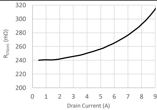
Figure 10. On-state resistance as a function of drain current at T_j = 25^\circ\text{C} .
