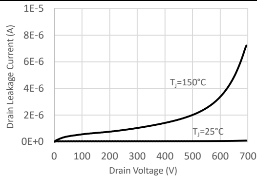
Figure 8. Drain leakage current characteristics at T_j = 25^\circ\text{C} and T_j = 150^\circ\text{C} .
