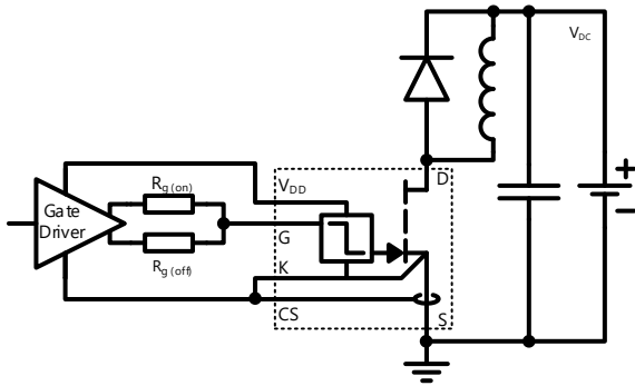
Figure 18. Inductive switching circuit. I_D = 6\text{ A} , R_{g(on)} = 15\ \Omega , R_{g(off)} = 2\ \Omega , V_{DD} = 12\text{ V} , V_{DC} = 400\text{ V} , L = 125\ \mu\text{H} , diode = IDH04G65C5.
