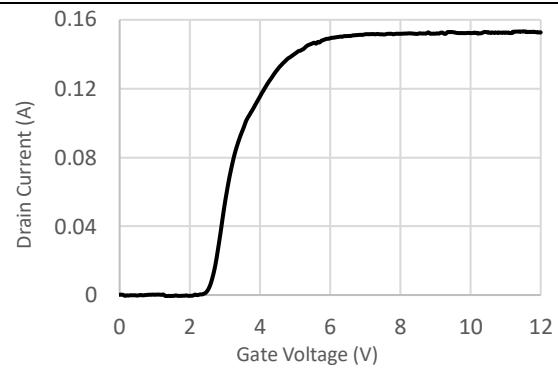
Figure 14. Transfer characteristics at V_{DS} = 0.1 \text{ V} , T_J = 150 \text{ }^{\circ}\text{C} .
