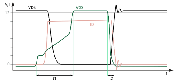
Figure 21. Q_G gate charge characterisation waveform at I_G = 15\text{ mA} and V_{DD} = 12\text{ V} . Time intervals t_1 and t_2 indicate the integration boundaries to calculate Q_G from I_G at turn-on and turn-off. Turn-off gate charge is lower than turn-on gate charge.
