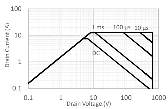
Figure 3. Safe Operating Area (SOA) based on thermal impedance Z_{thJC} at T_{CASE} = 25\text{ }^{\circ}\text{C} .
