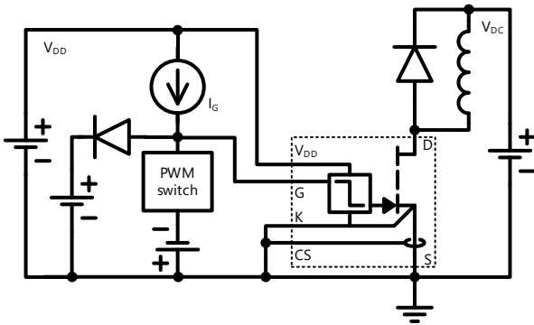
Figure 20. Q_G gate charge characterization circuit. I_G = 15\text{ mA} , V_{DC} = 400\text{ V} , V_{DD} = 12\text{ V} , L = 125\ \mu\text{H} , freewheeling diode = IDH04G65C5.
